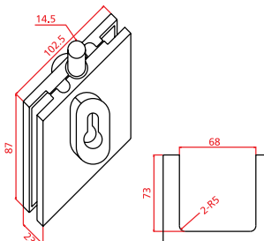
CK-060 Kilit Lock
