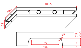
CK-040 Cam Cama Menteşe Glass to Glass Hinge
